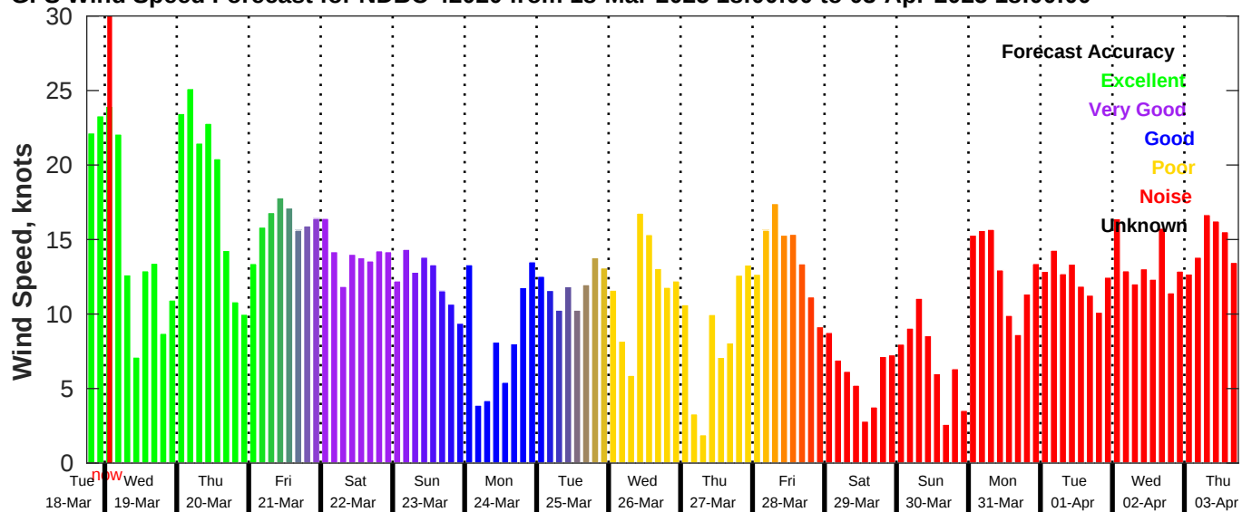
GFS Wind Speed Forecast for NDBC 42020 from 18-Mar-2025 18:00:00 to 03-Apr-2025 18:00:00
