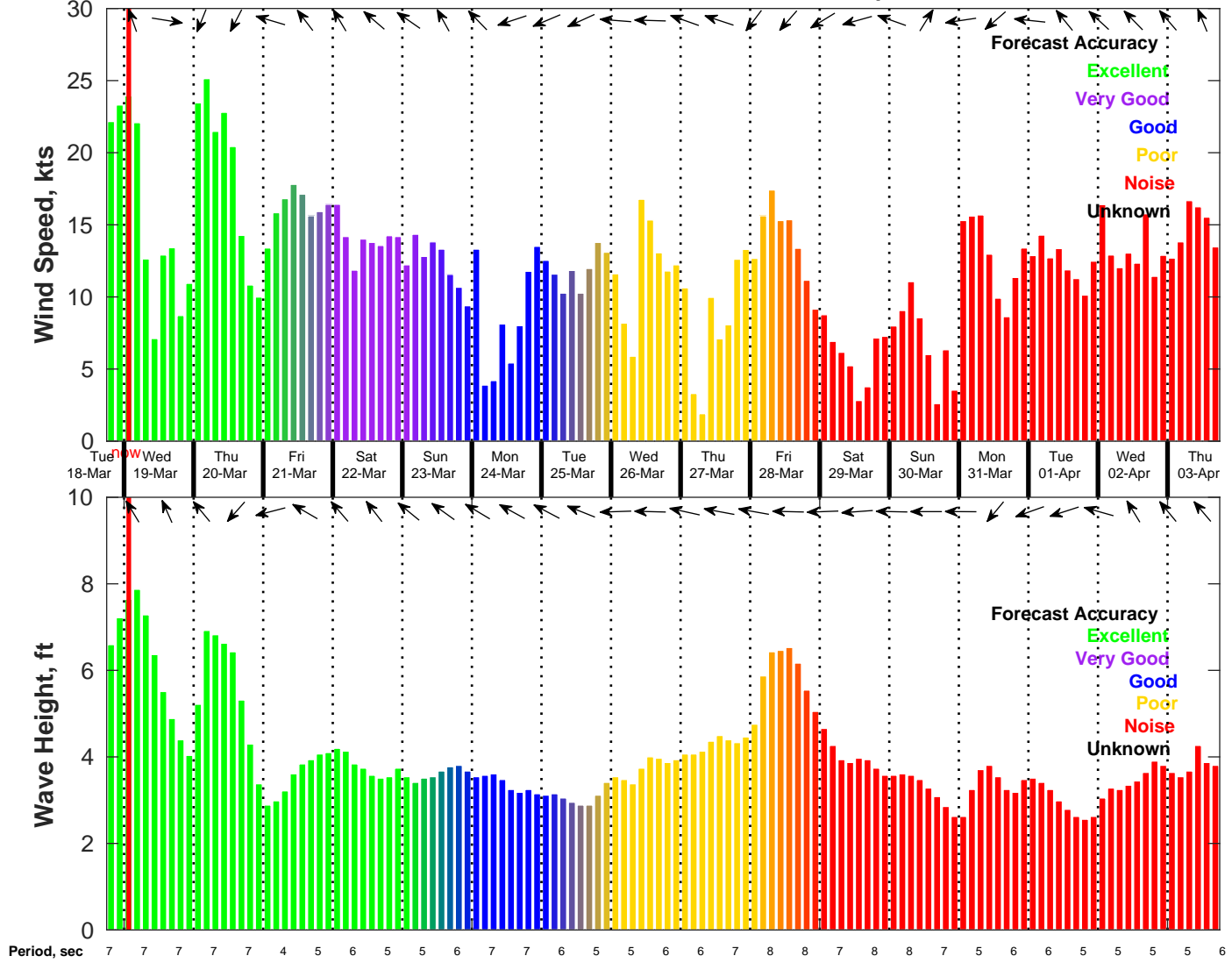
Wind & Wave Forecast for NDBC 42020 from 18-Mar-2025 18:00:00 to 03-Apr-2025 18:00:00
