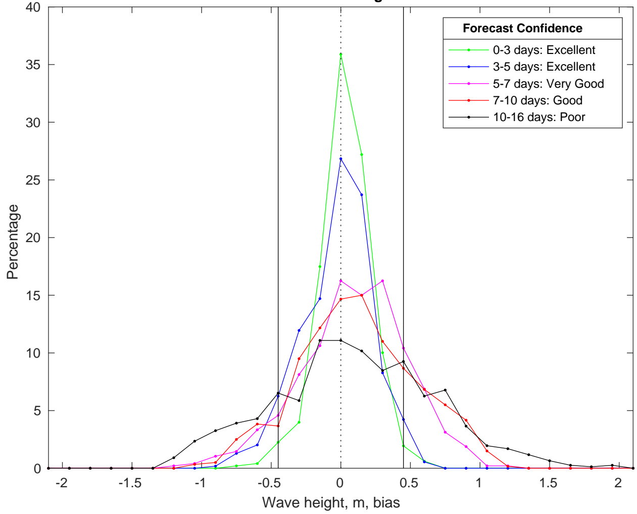
NDBC 42035 vs GFS Waves Bias Histogram: 19-Mar-2025
