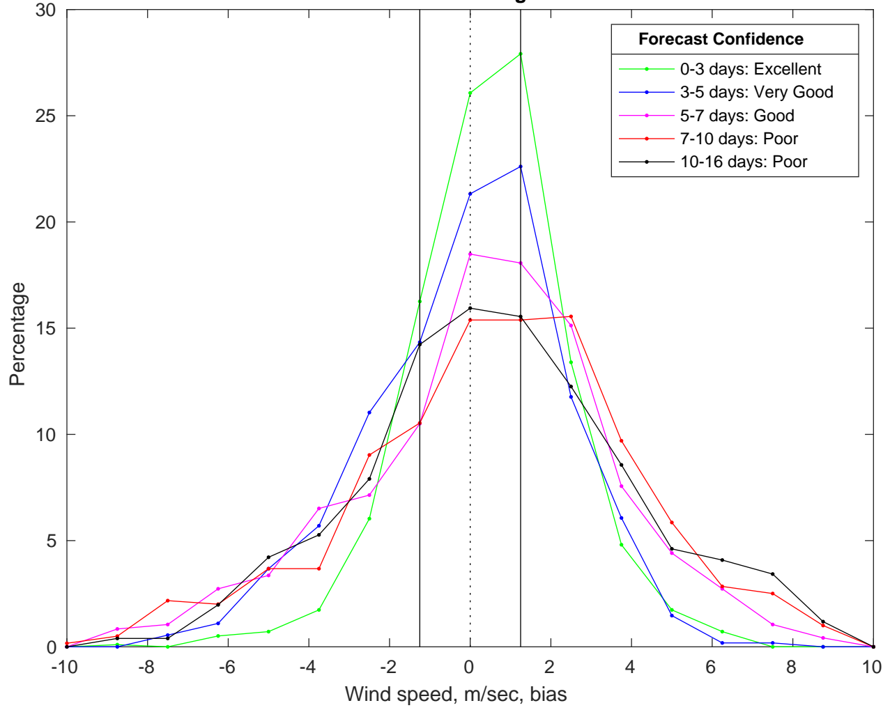
NDBC 42035 vs GFS Winds Bias Histogram: 19-Mar-2025
