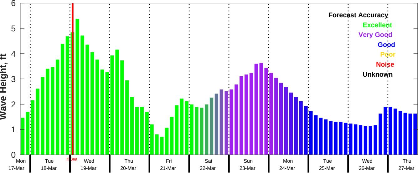
CMEMS Wave Forecast for NDBC 42035 from 17-Mar-2025 18:00:00 to 27-Mar-2025 18:00:00
