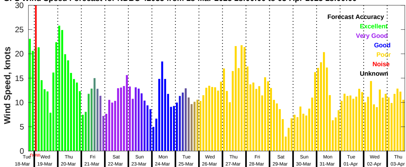
GFS Wind Speed Forecast for NDBC 42035 from 18-Mar-2025 18:00:00 to 03-Apr-2025 18:00:00
