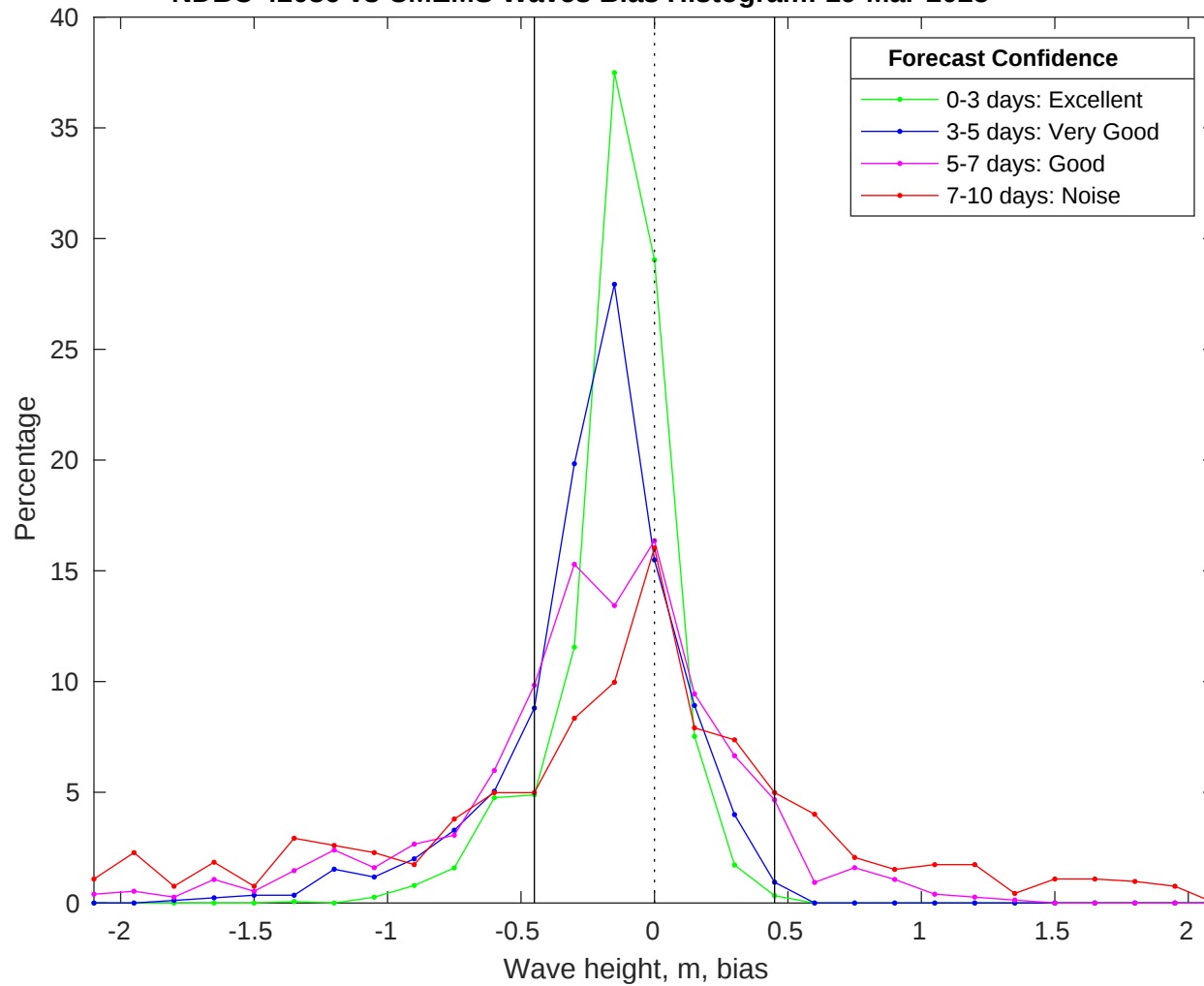
NDBC 42036 vs CMEMS Waves Bias Histogram: 19-Mar-2025
