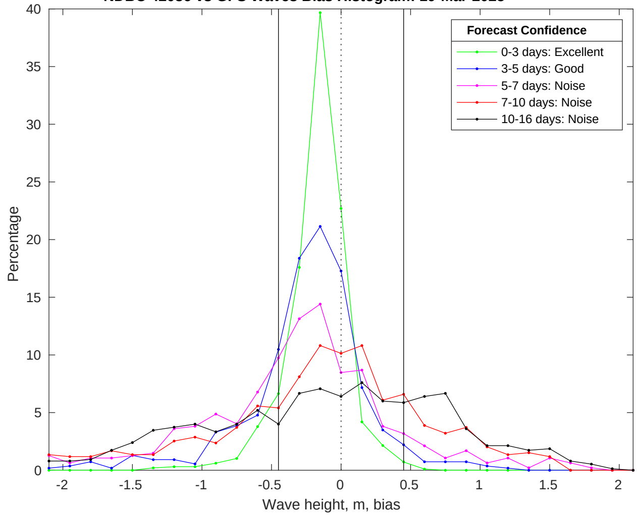
NDBC 42036 vs GFS Waves Bias Histogram: 19-Mar-2025
