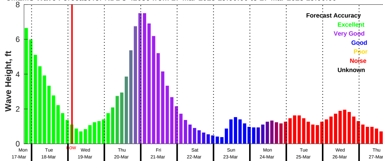
CMEMS Wave Forecast for NDBC 42036 from 17-Mar-2025 19:00:00 to 27-Mar-2025 19:00:00
