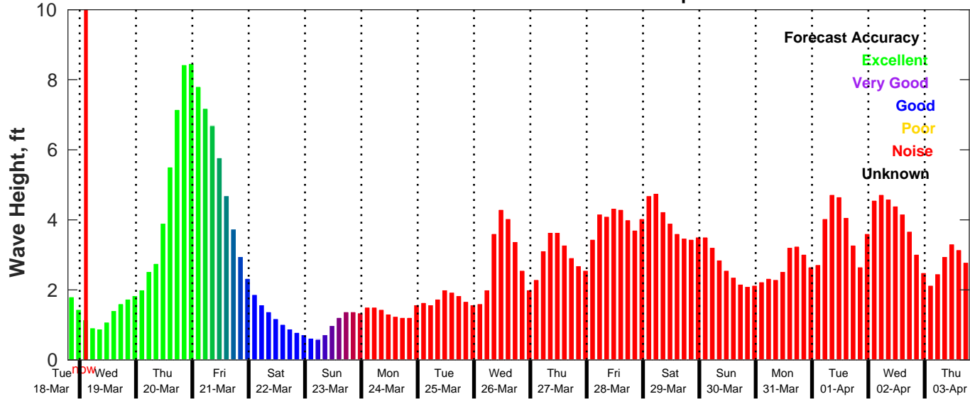
GFS Wave Forecast for NDBC 42036 from 18-Mar-2025 19:00:00 to 03-Apr-2025 19:00:00
