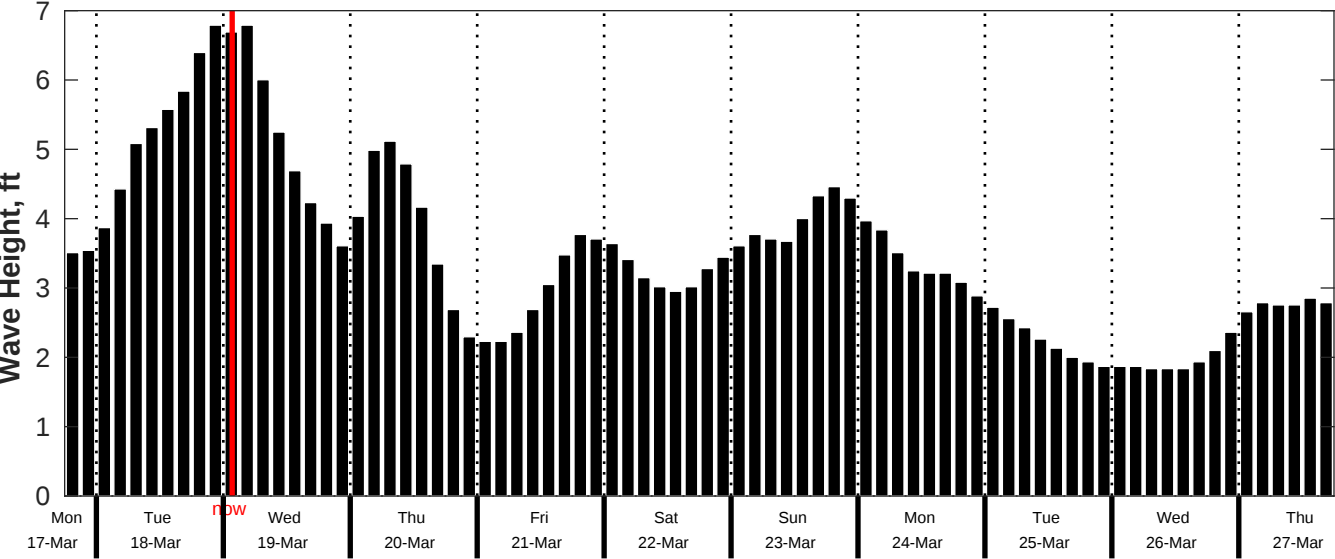
CMEMS Wave Forecast for NDBC 42092 from 17-Mar-2025 18:00:00 to 27-Mar-2025 18:00:00
