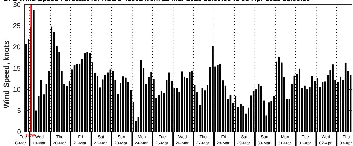
GFS Wind Speed Forecast for NDBC 42092 from 18-Mar-2025 18:00:00 to 03-Apr-2025 18:00:00
