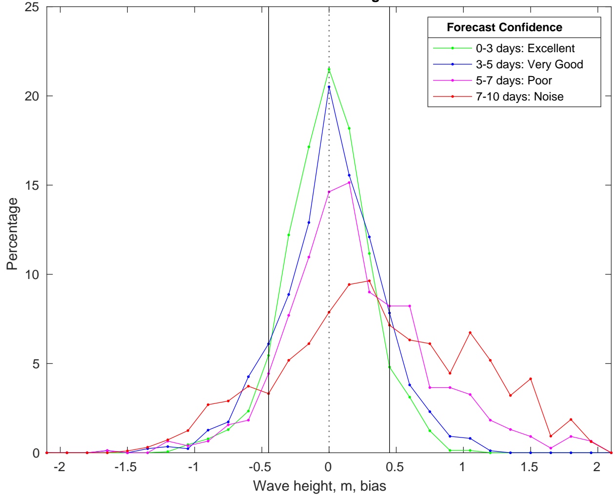
NDBC 46011 vs CMEMS Waves Bias Histogram: 19-Mar-2025
