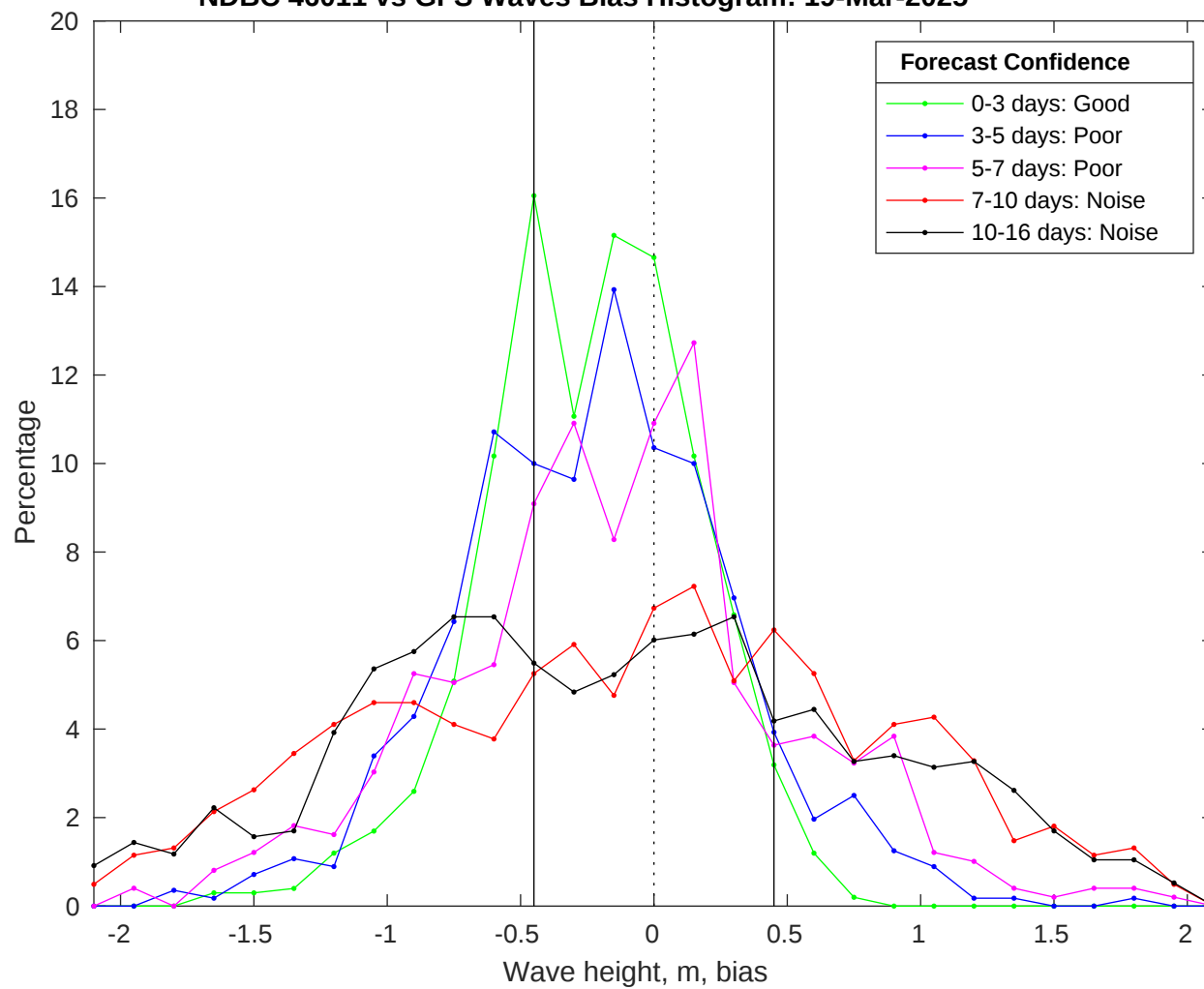
NDBC 46011 vs GFS Waves Bias Histogram: 19-Mar-2025
