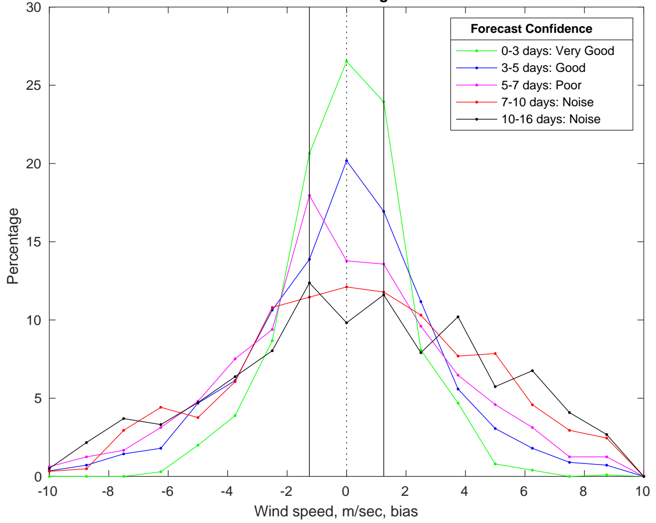
NDBC 46011 vs GFS Winds Bias Histogram: 19-Mar-2025
