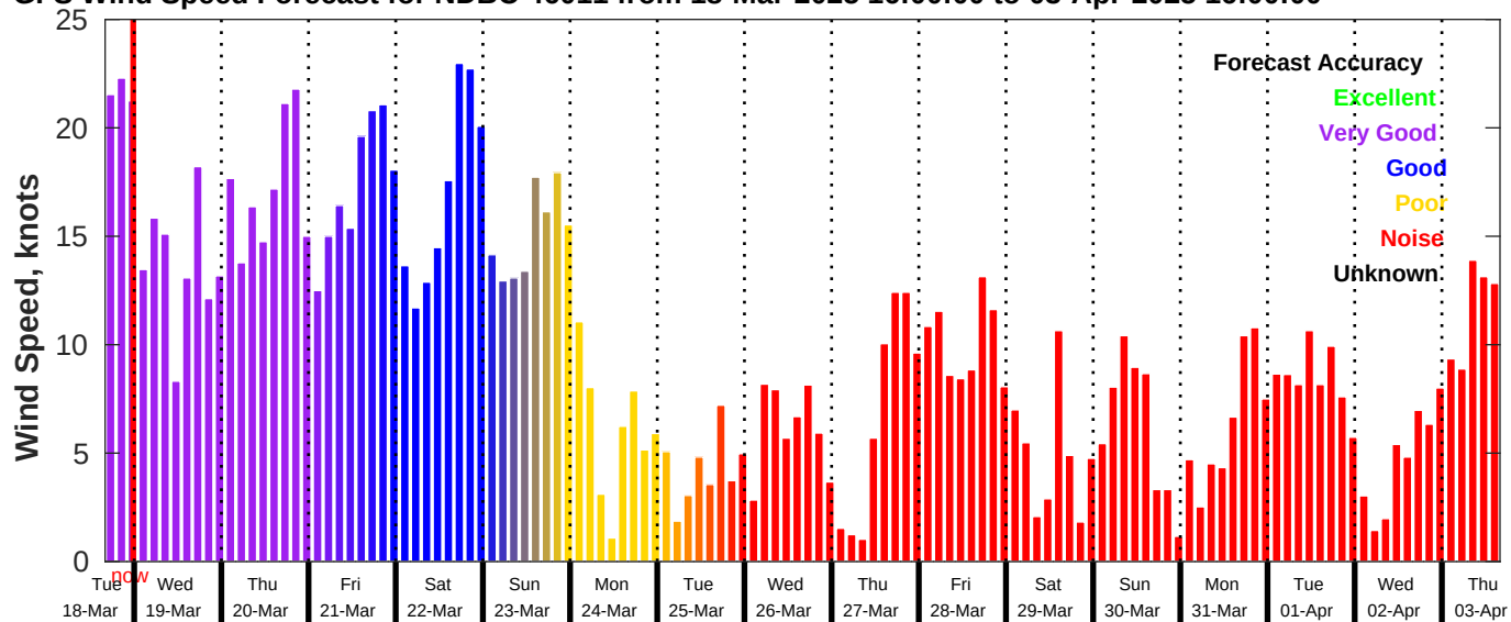
GFS Wind Speed Forecast for NDBC 46011 from 18-Mar-2025 16:00:00 to 03-Apr-2025 16:00:00
