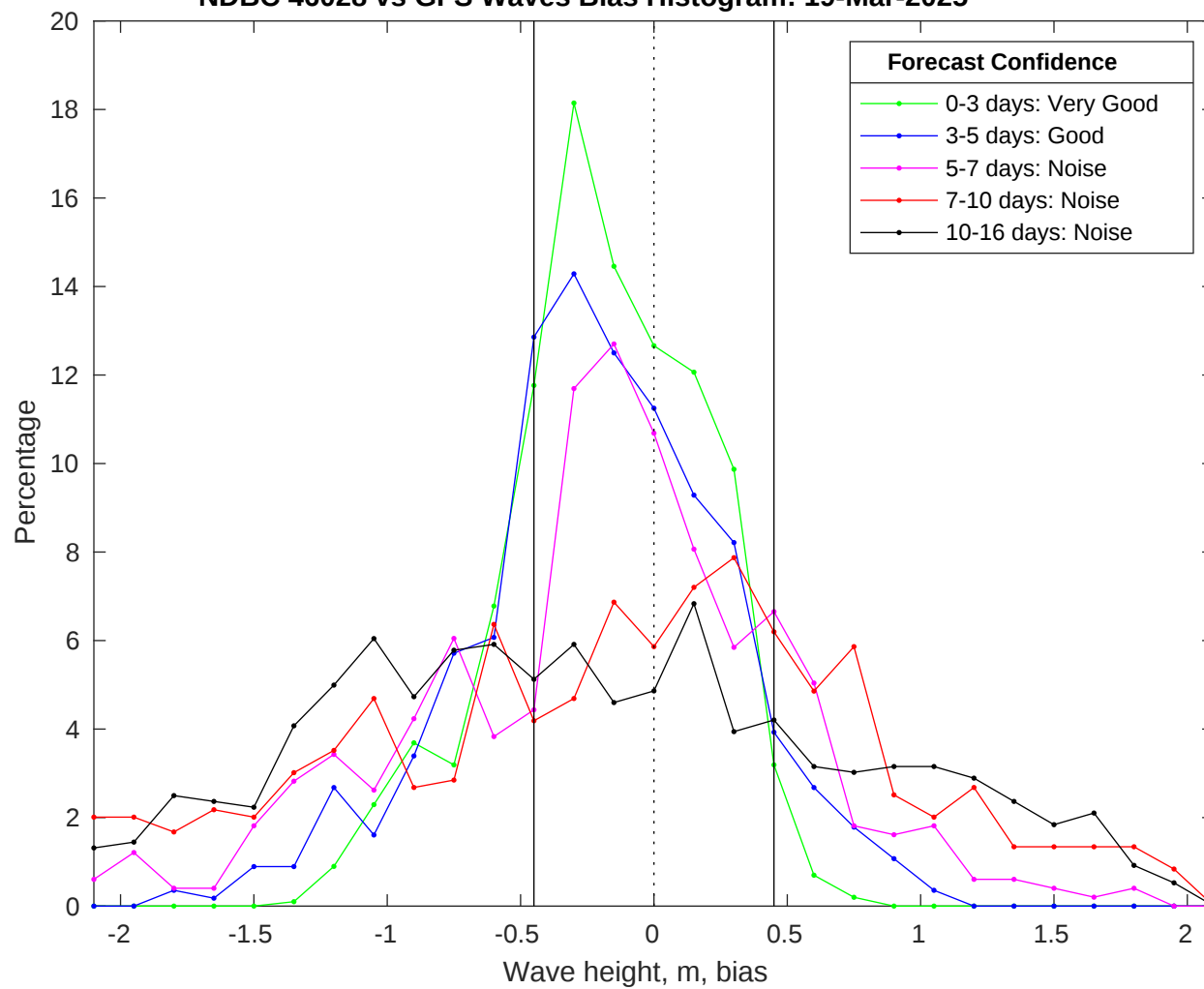
NDBC 46028 vs GFS Waves Bias Histogram: 19-Mar-2025
