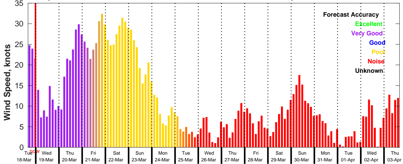
GFS Wind Speed Forecast for NDBC 46028 from 18-Mar-2025 16:00:00 to 03-Apr-2025 16:00:00
