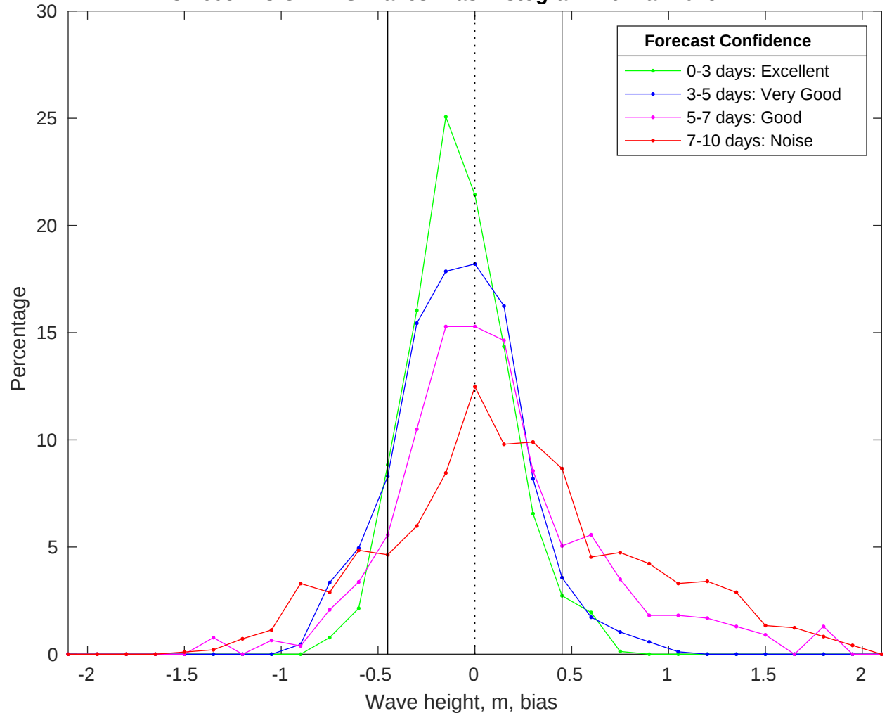
NDBC 46054 vs CMEMS Waves Bias Histogram: 19-Mar-2025
