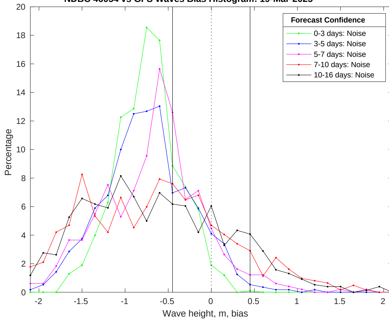
NDBC 46054 vs GFS Waves Bias Histogram: 19-Mar-2025
