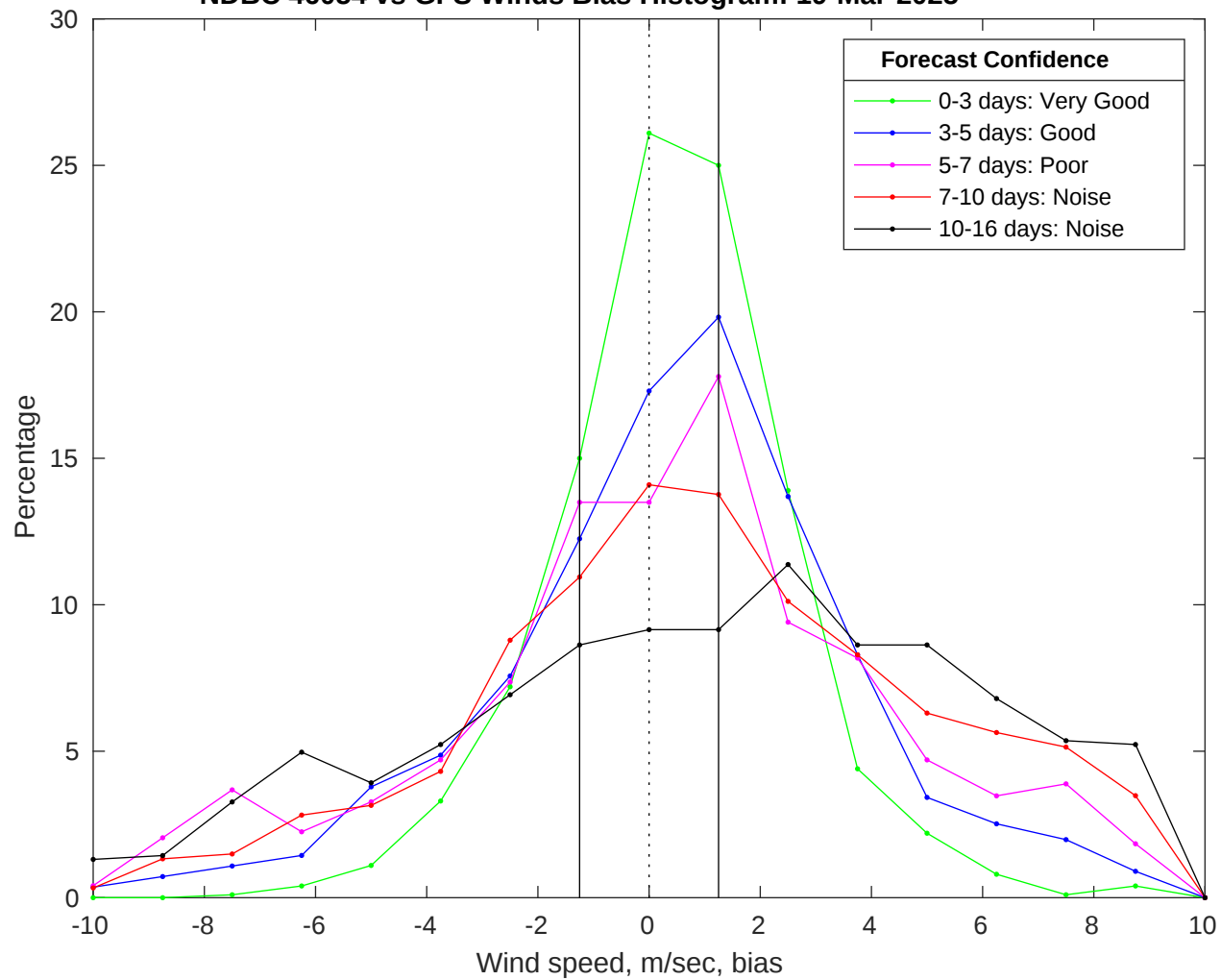
NDBC 46054 vs GFS Winds Bias Histogram: 19-Mar-2025
