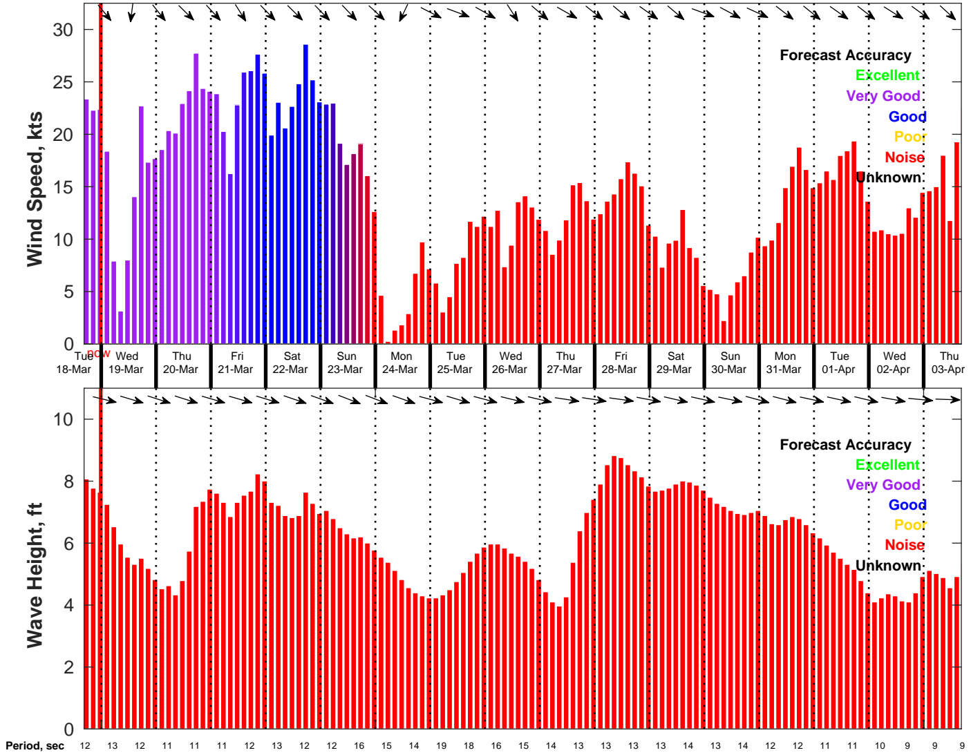
Wind & Wave Forecast for NDBC 46054 from 18-Mar-2025 16:00:00 to 03-Apr-2025 16:00:00
