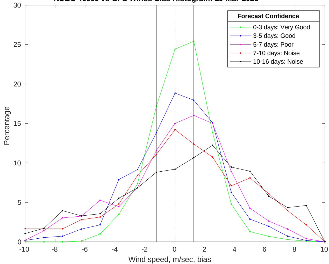
NDBC 46069 vs GFS Winds Bias Histogram: 19-Mar-2025
