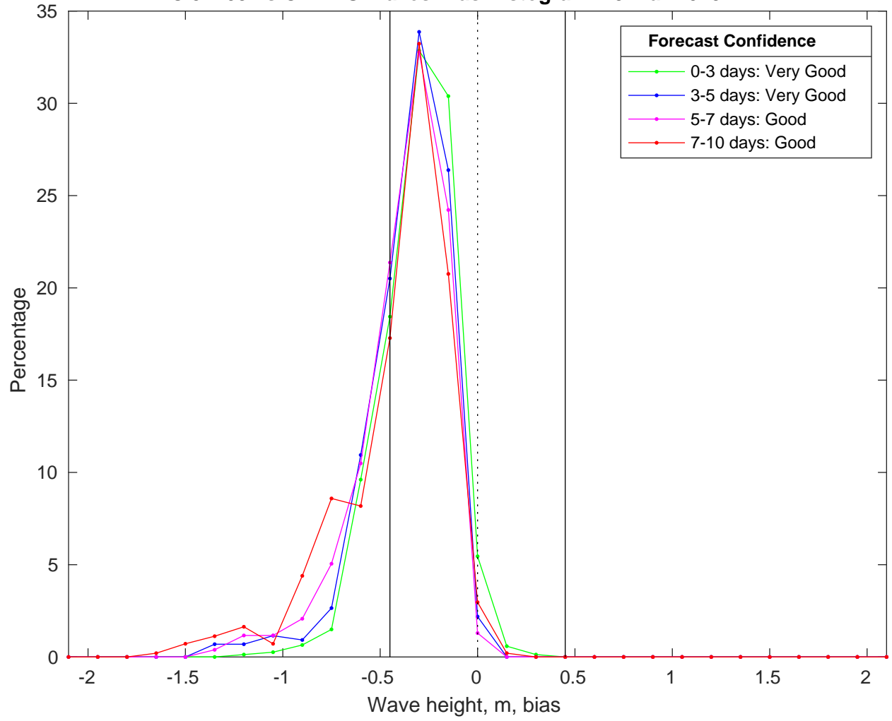
NDBC 51209 vs CMEMS Waves Bias Histogram: 19-Mar-2025
