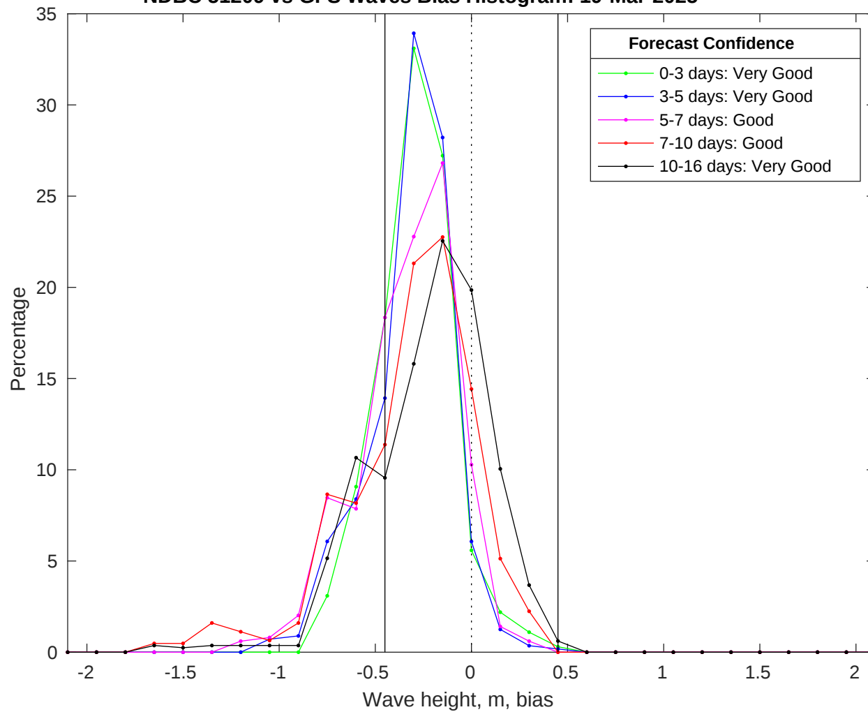
NDBC 51209 vs GFS Waves Bias Histogram: 19-Mar-2025
