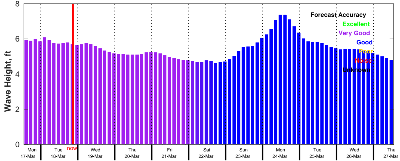
CMEMS Wave Forecast for NDBC 51209 from 17-Mar-2025 13:00:00 to 27-Mar-2025 13:00:00
