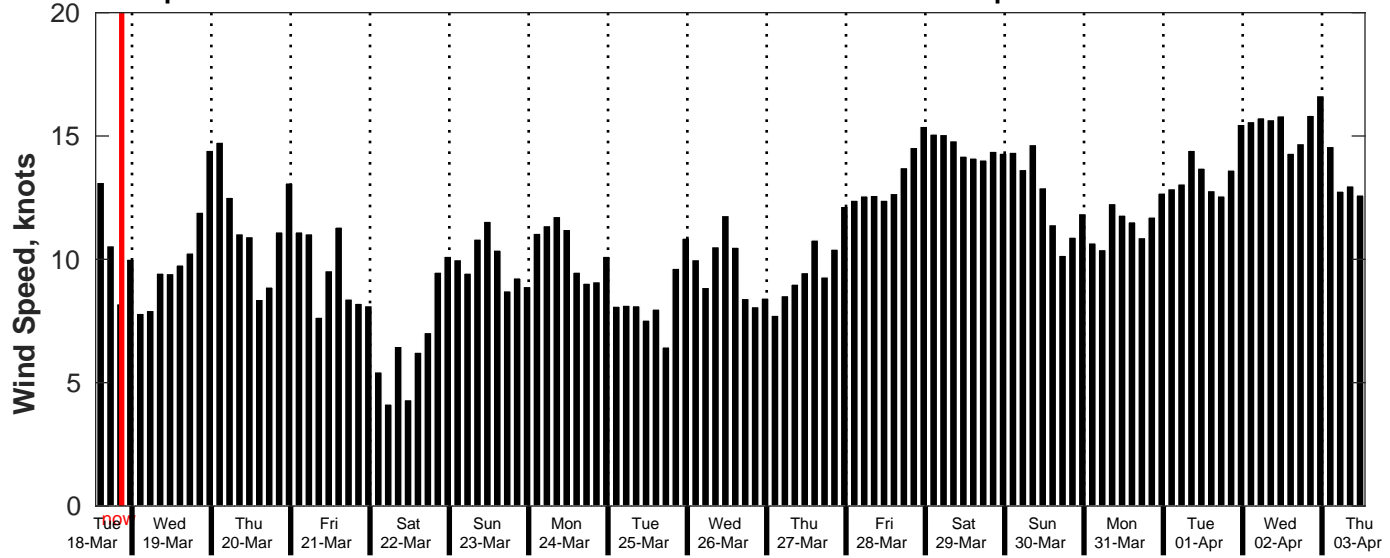
GFS Wind Speed Forecast for NDBC 51209 from 18-Mar-2025 13:00:00 to 03-Apr-2025 13:00:00
