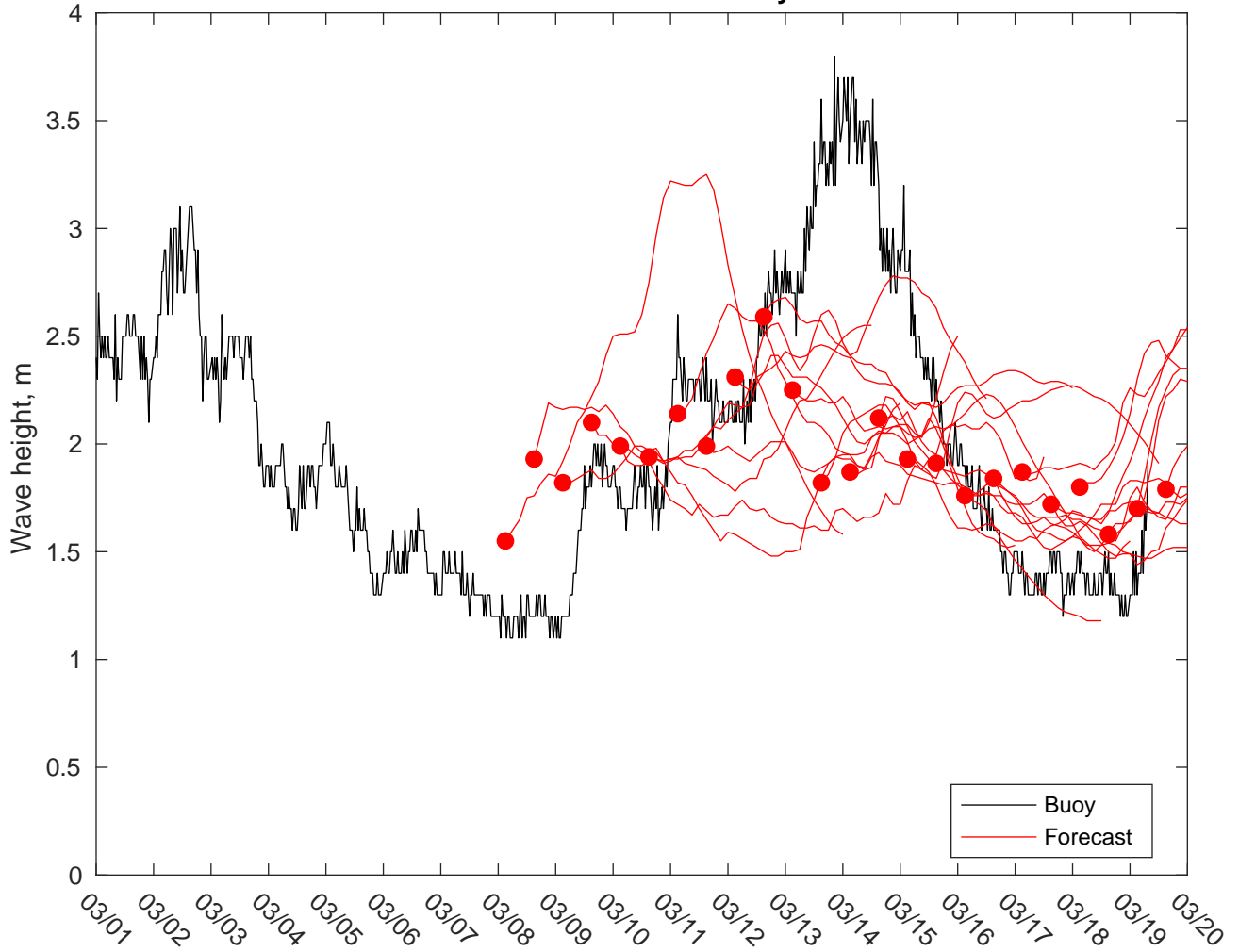
NDBC 52211 vs GFS Waves: 10 to 16 day forecast
