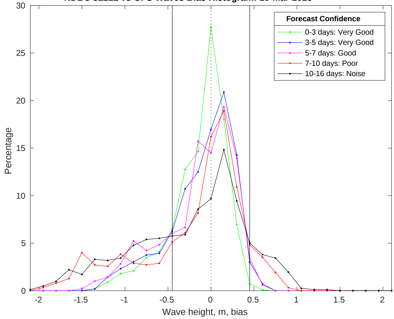
NDBC 52211 vs GFS Waves Bias Histogram: 19-Mar-2025
