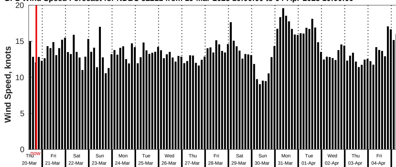
GFS Wind Speed Forecast for NDBC 52211 from 19-Mar-2025 10:00:00 to 04-Apr-2025 10:00:00
