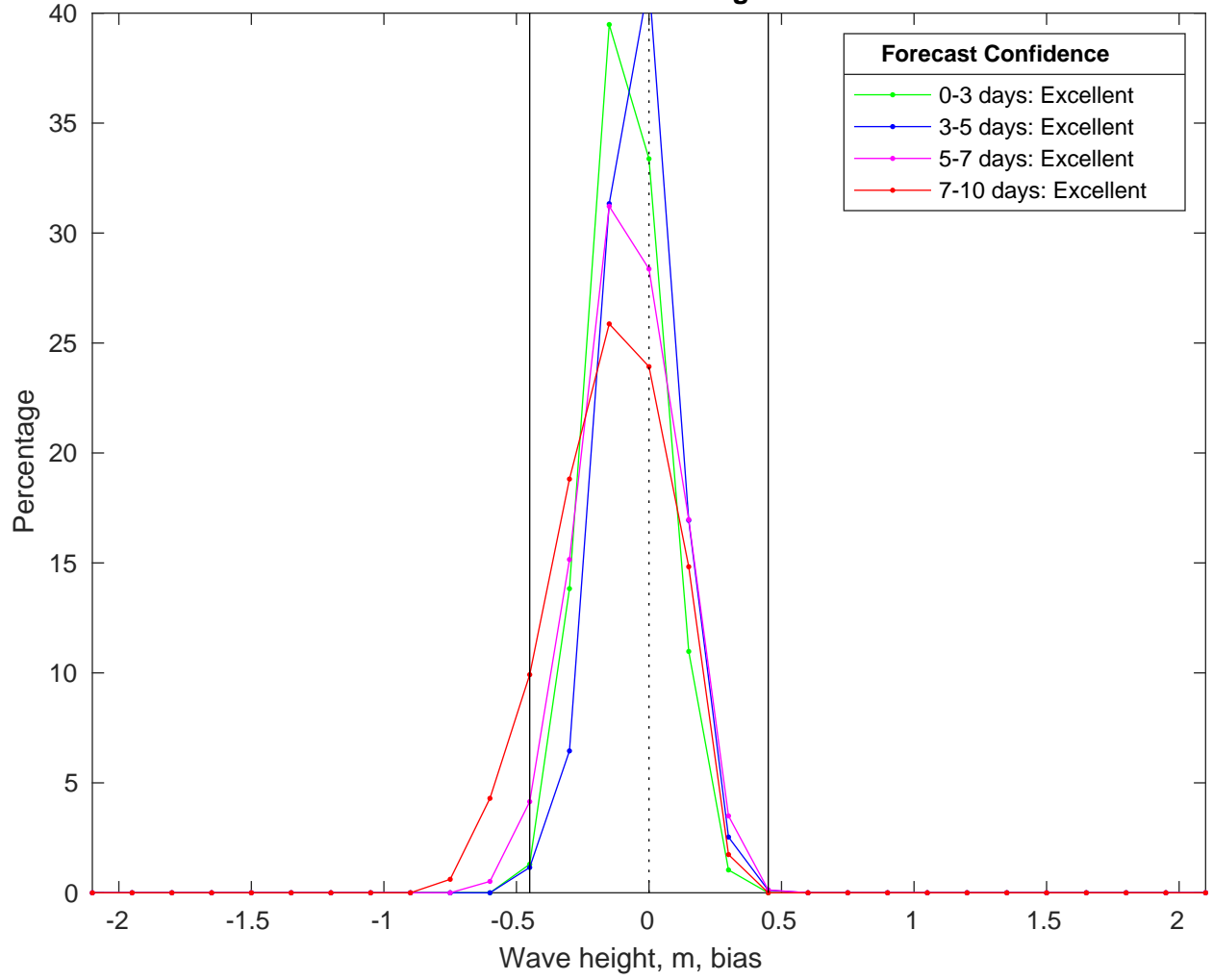
NDBC 52212 vs CMEMS Waves Bias Histogram: 19-Mar-2025
