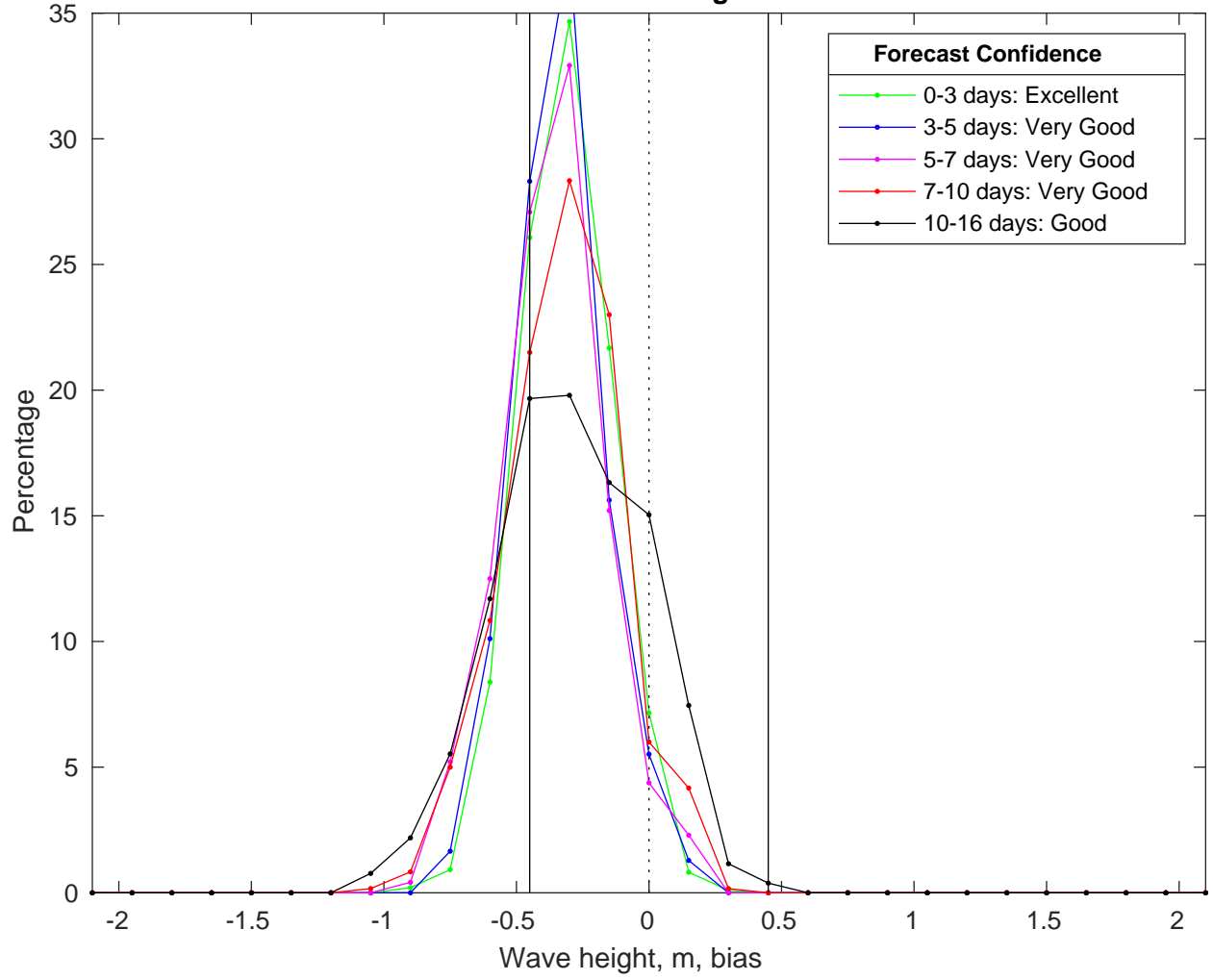
NDBC 52212 vs GFS Waves Bias Histogram: 19-Mar-2025
