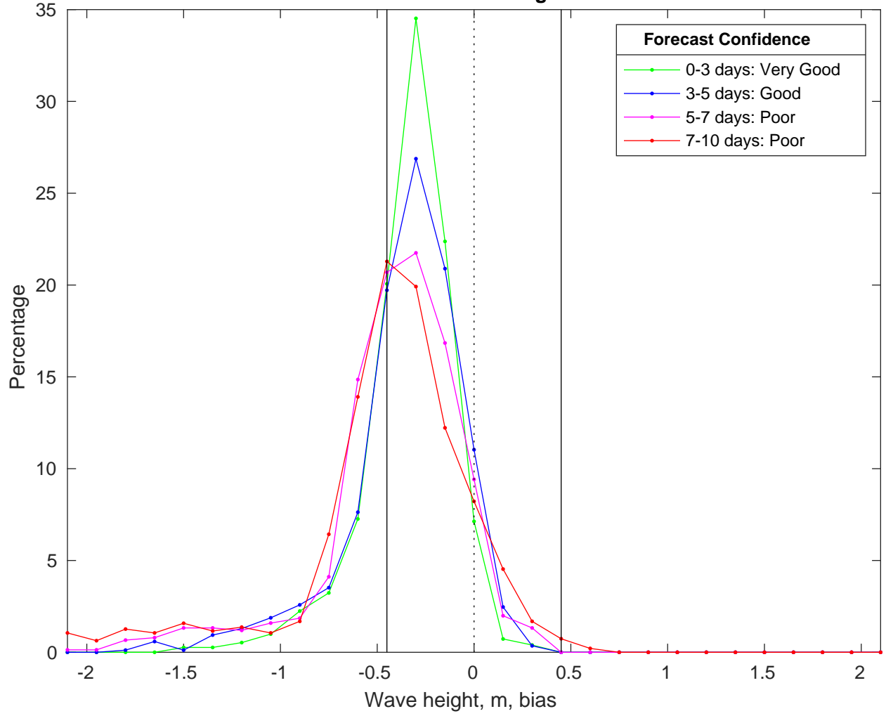
NDBC 52213 vs CMEMS Waves Bias Histogram: 19-Mar-2025
