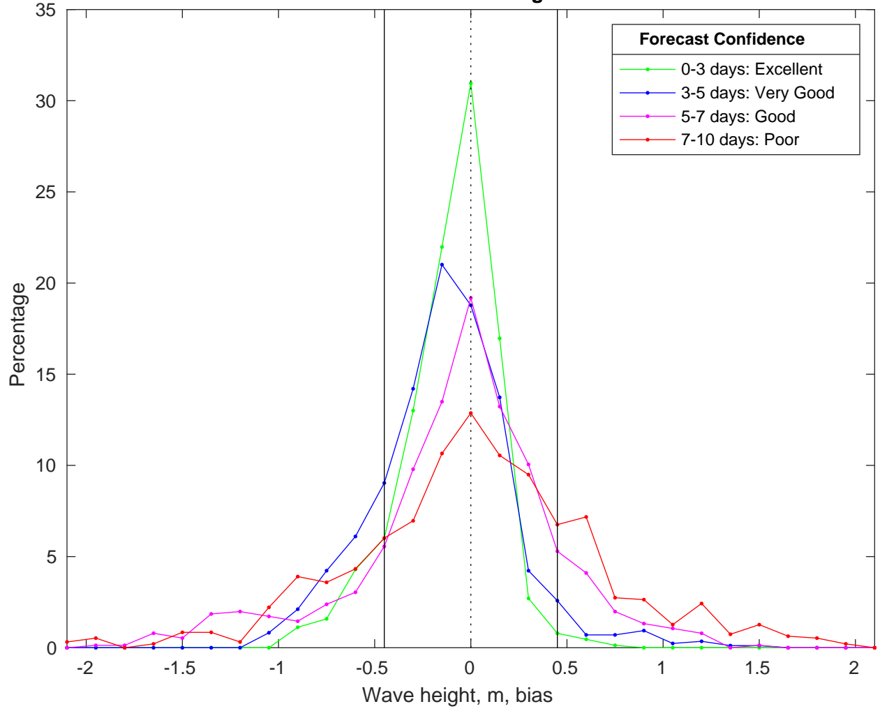
NDBC 41004 vs CMEMS Waves Bias Histogram: 20-Mar-2025
