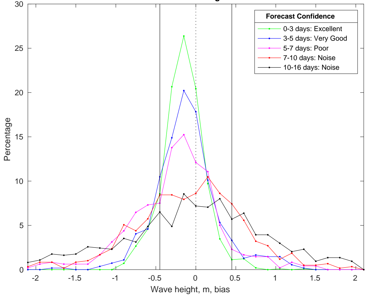
NDBC 41004 vs GFS Waves Bias Histogram: 20-Mar-2025
