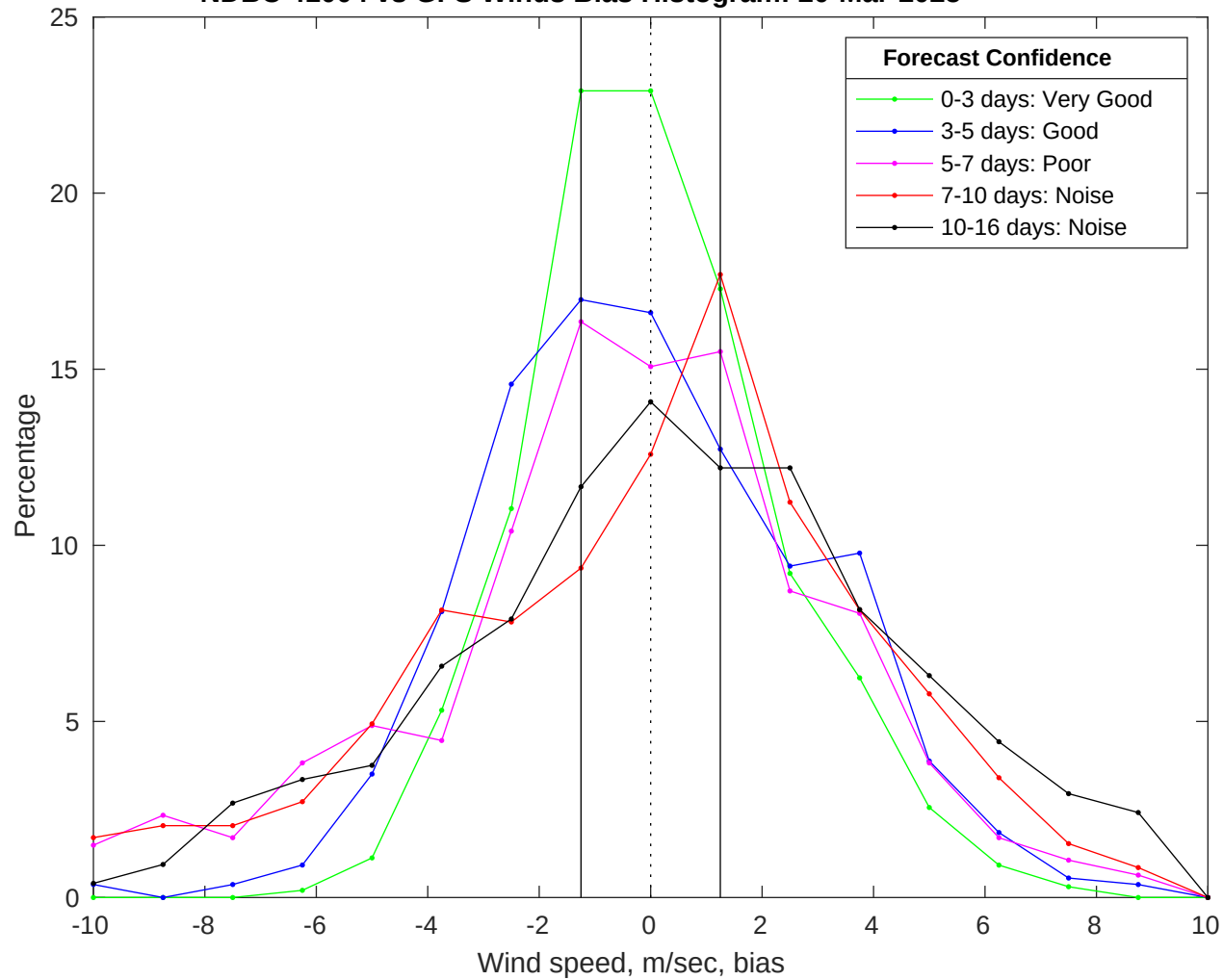
NDBC 41004 vs GFS Winds Bias Histogram: 20-Mar-2025
