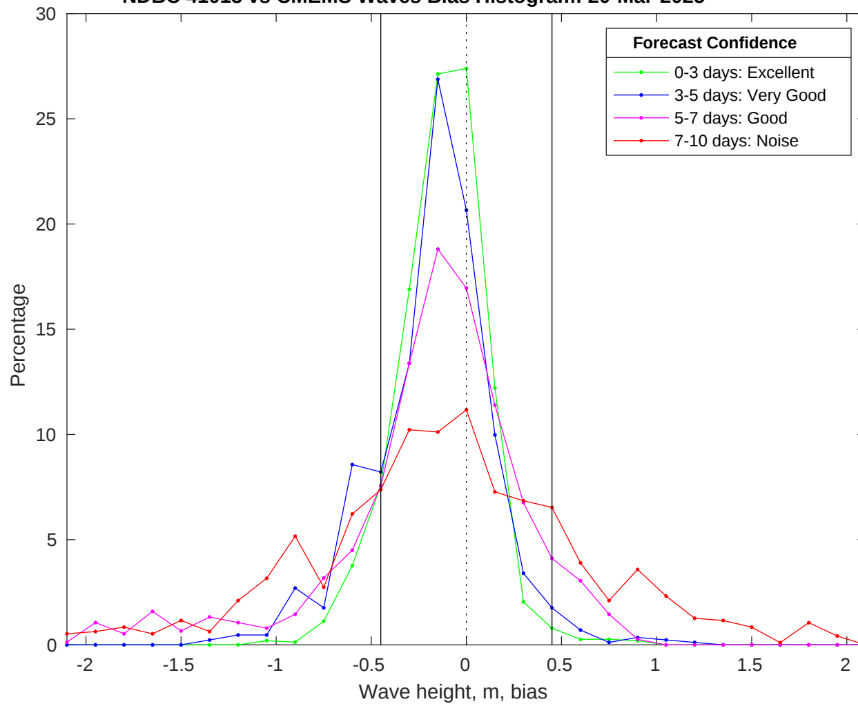
NDBC 41013 vs CMEMS Waves Bias Histogram: 20-Mar-2025
