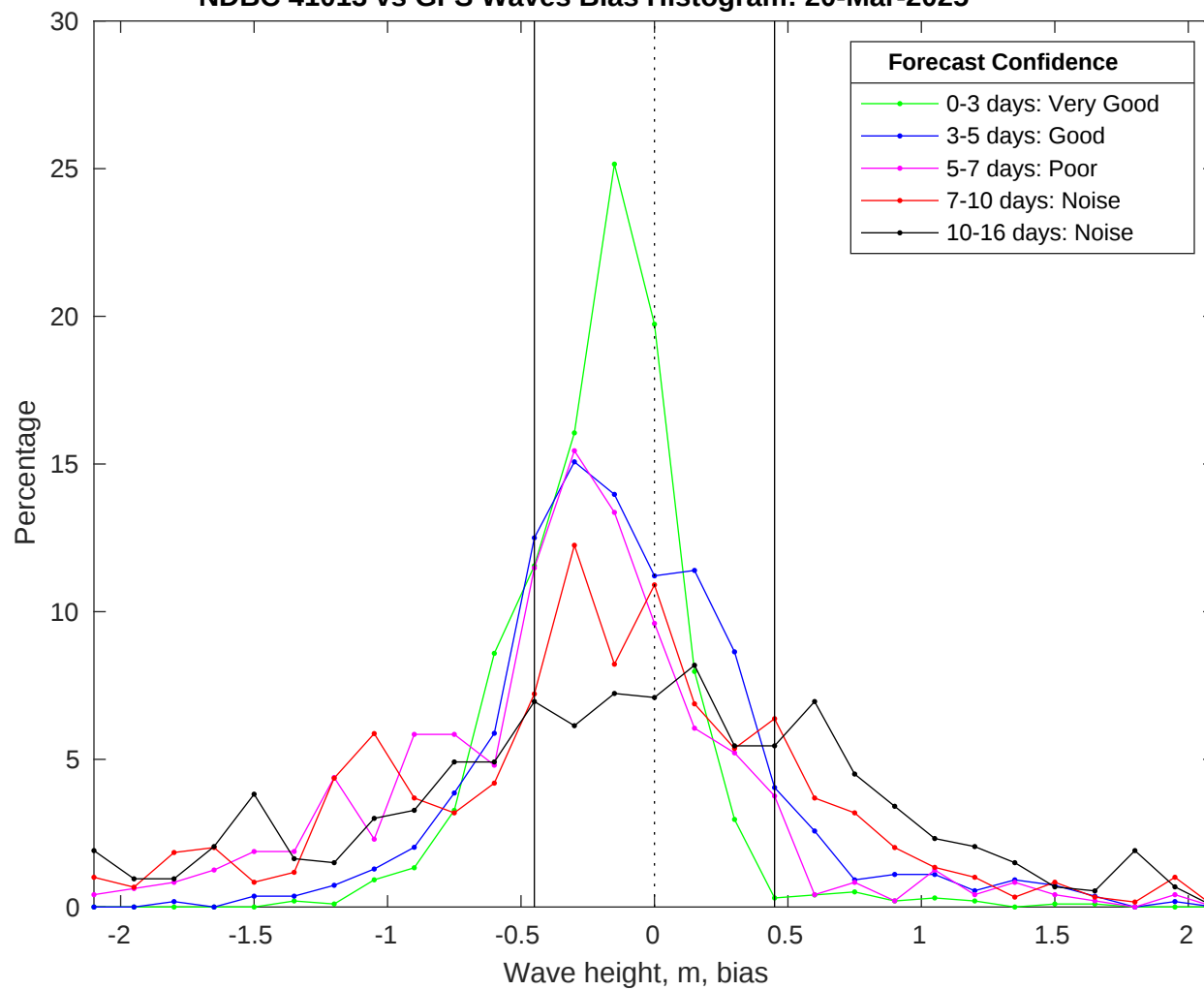
NDBC 41013 vs GFS Waves Bias Histogram: 20-Mar-2025
