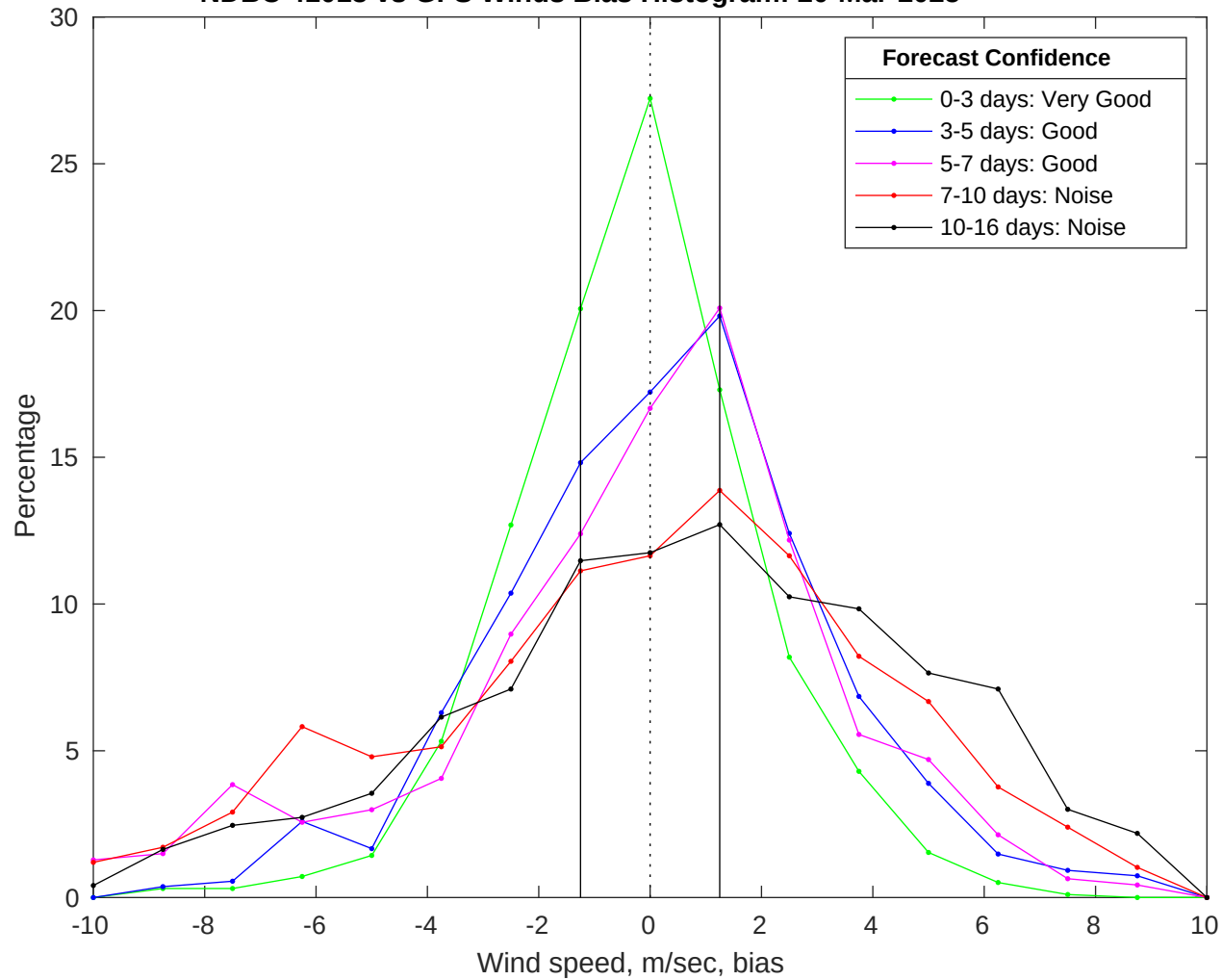
NDBC 41013 vs GFS Winds Bias Histogram: 20-Mar-2025
