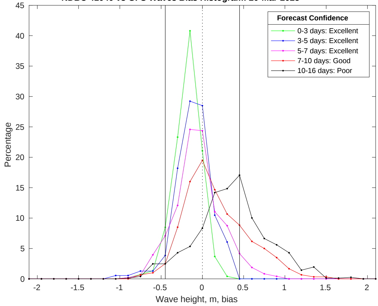
NDBC 41040 vs GFS Waves Bias Histogram: 20-Mar-2025
