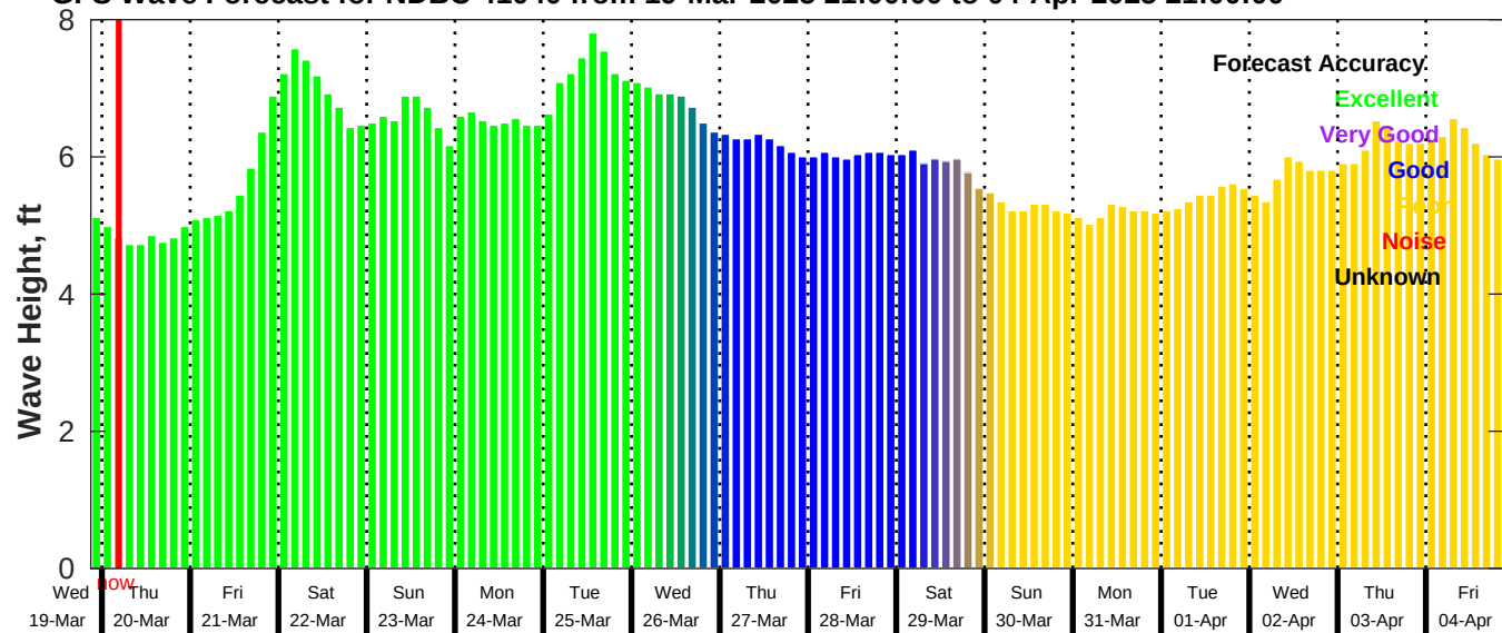
GFS Wave Forecast for NDBC 41040 from 19-Mar-2025 21:00:00 to 04-Apr-2025 21:00:00
