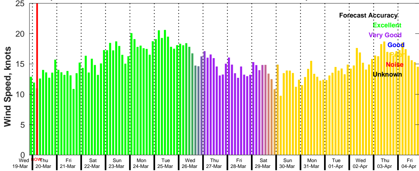
GFS Wind Speed Forecast for NDBC 41040 from 19-Mar-2025 21:00:00 to 04-Apr-2025 21:00:00
