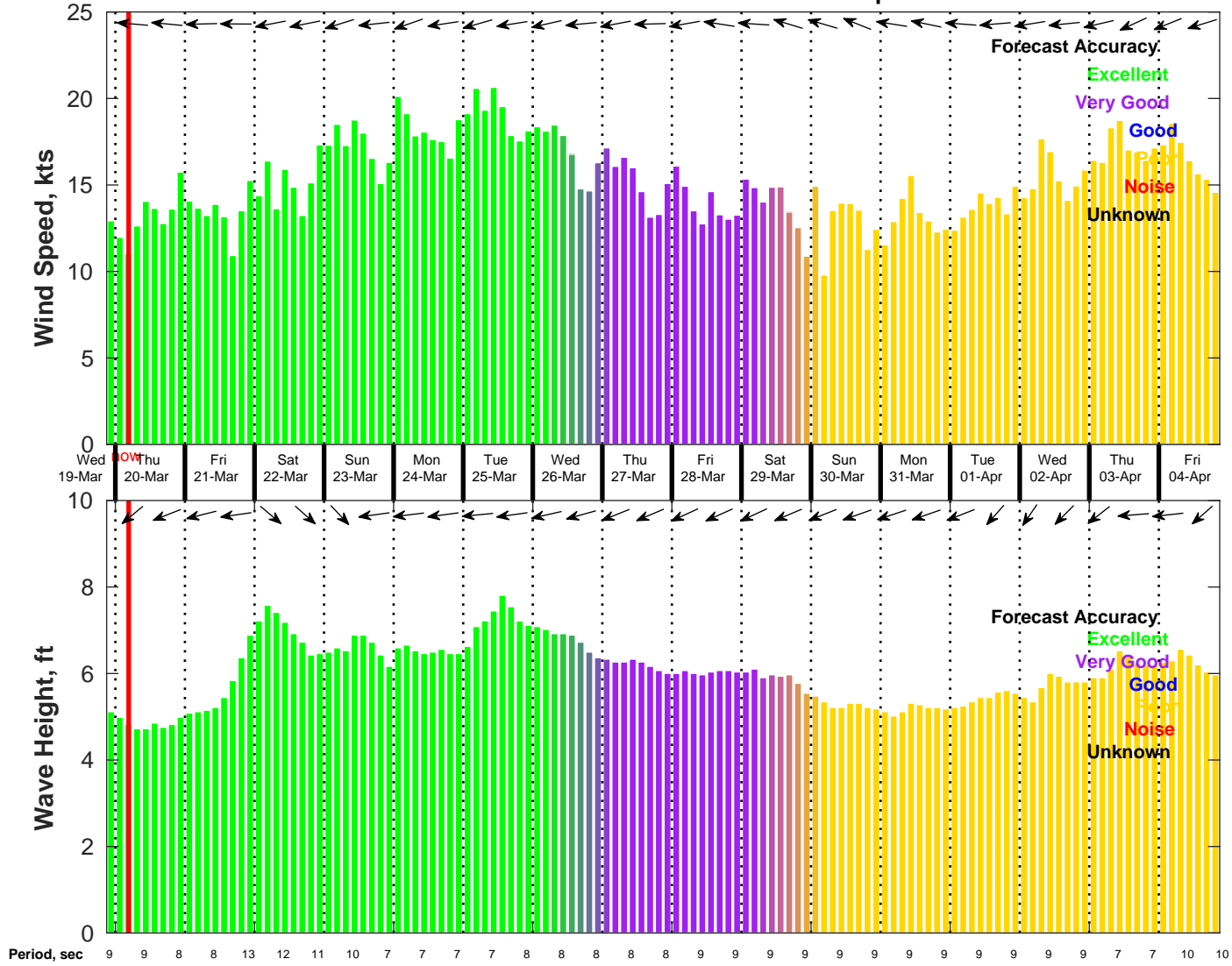
Wind & Wave Forecast for NDBC 41040 from 19-Mar-2025 21:00:00 to 04-Apr-2025 21:00:00
