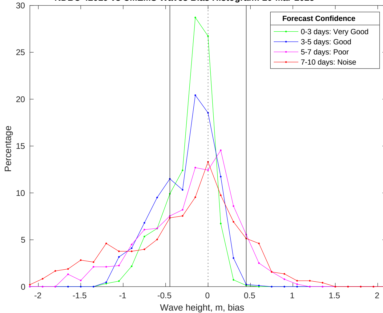
NDBC 42019 vs CMEMS Waves Bias Histogram: 20-Mar-2025
