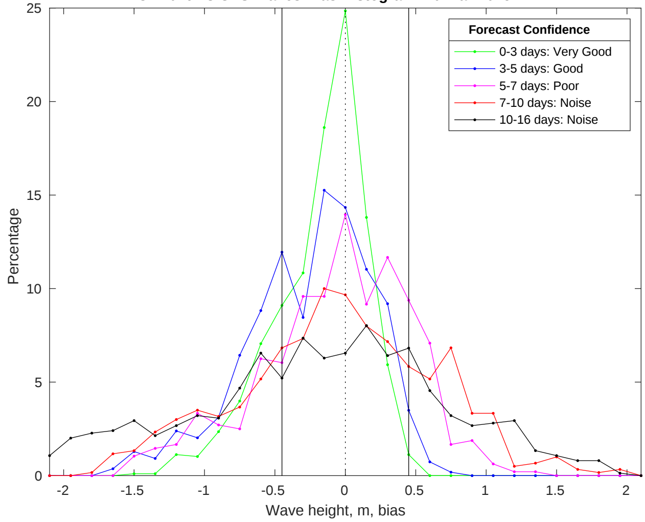
NDBC 42019 vs GFS Waves Bias Histogram: 20-Mar-2025
