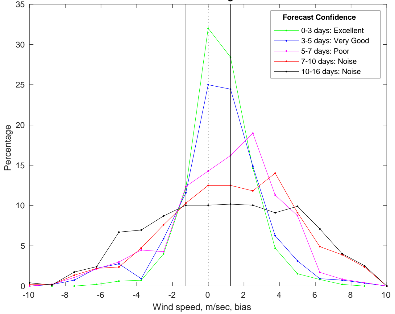
NDBC 42019 vs GFS Winds Bias Histogram: 20-Mar-2025
