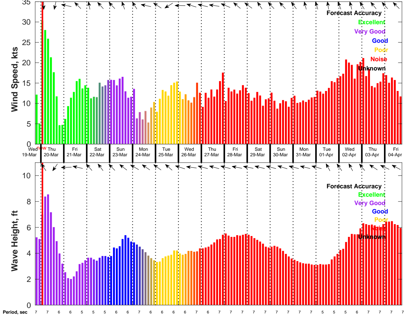
Wind & Wave Forecast for NDBC 42019 from 19-Mar-2025 18:00:00 to 04-Apr-2025 18:00:00
