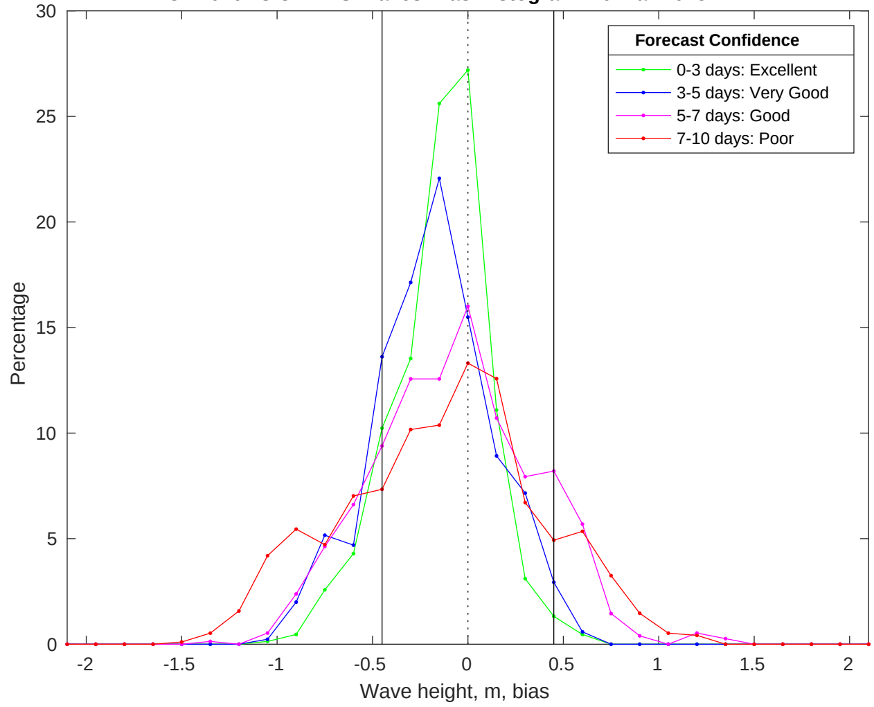
NDBC 42020 vs CMEMS Waves Bias Histogram: 20-Mar-2025
