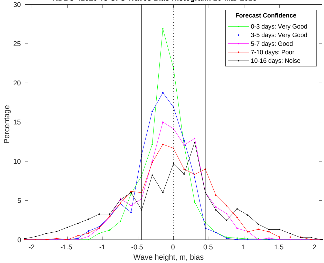
NDBC 42020 vs GFS Waves Bias Histogram: 20-Mar-2025
