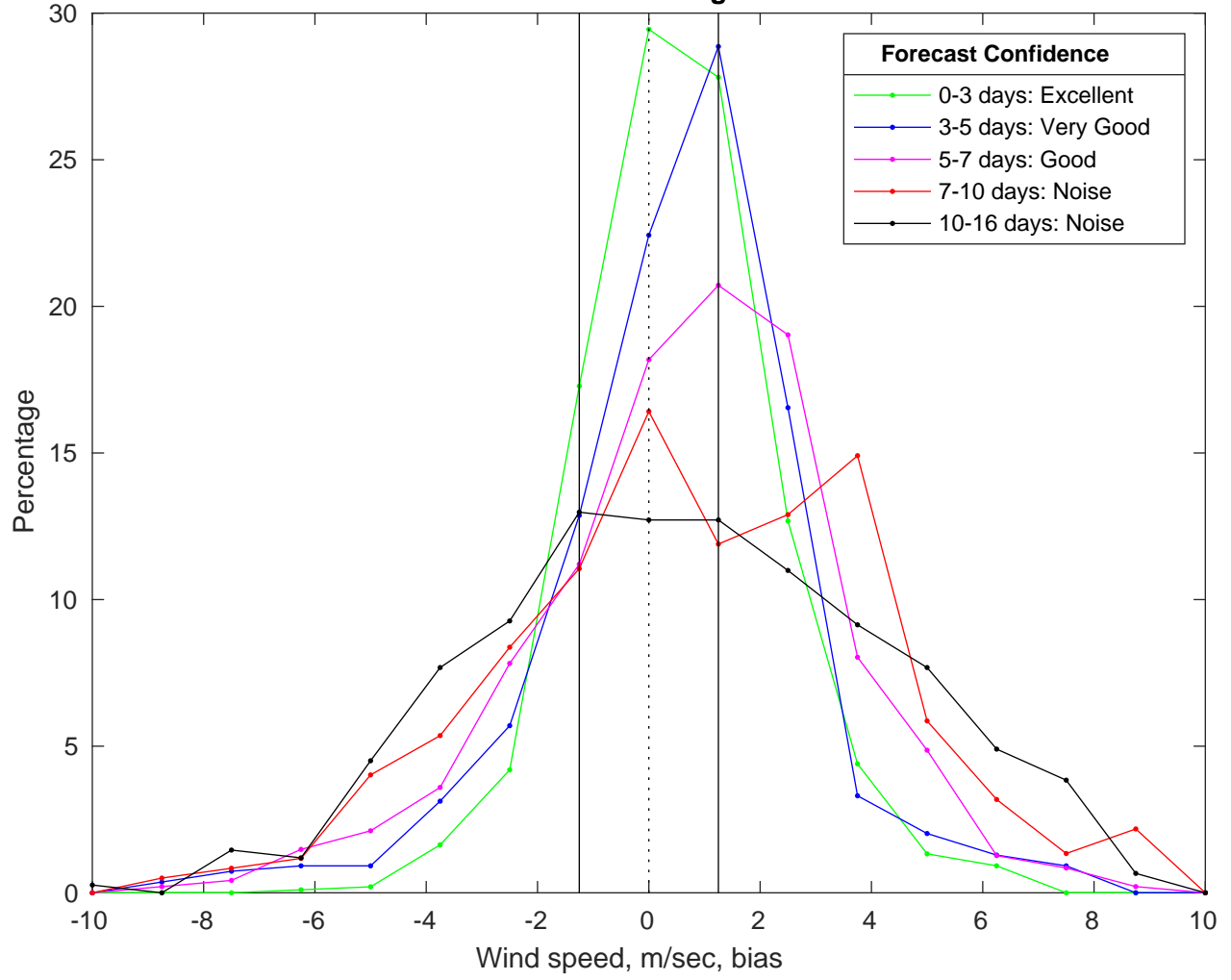
NDBC 42020 vs GFS Winds Bias Histogram: 20-Mar-2025
